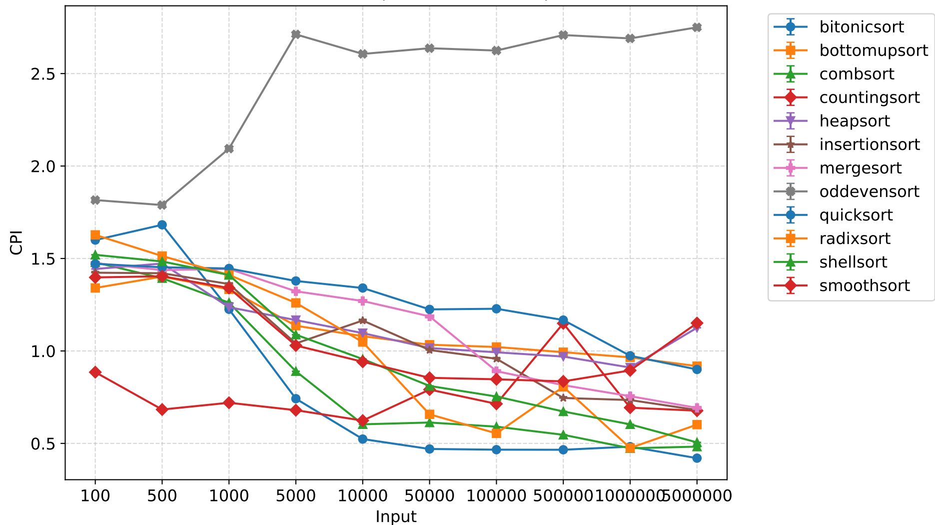
CPI - 1 thread (mean \pm 95% CI)
