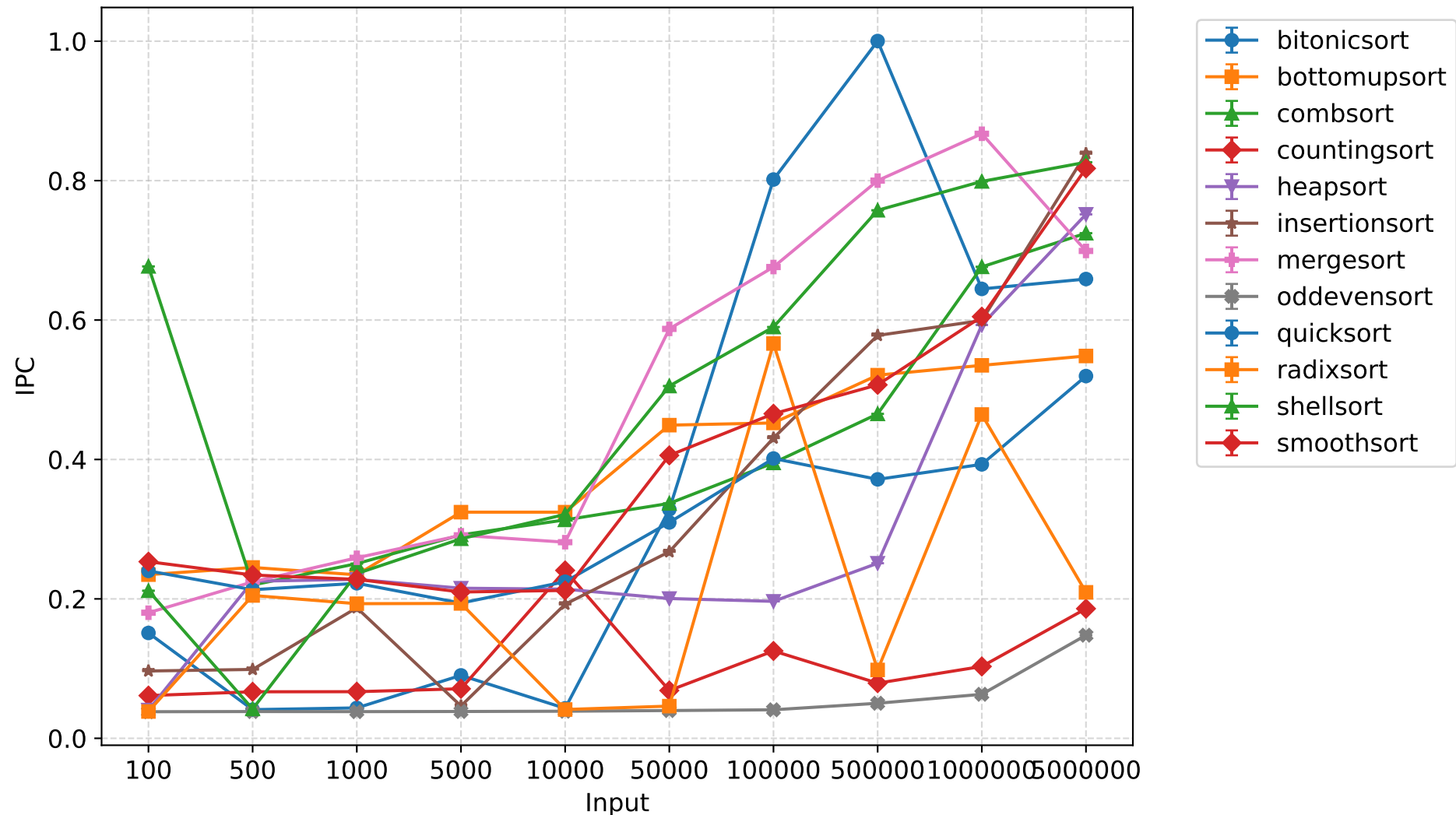
IPC - 8 threads (mean \pm 95% CI)
