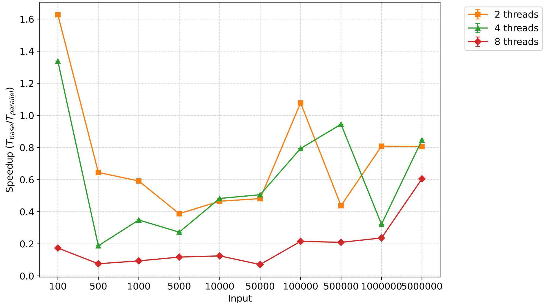
Speedup - counting sort (mean \pm 95% CI)
