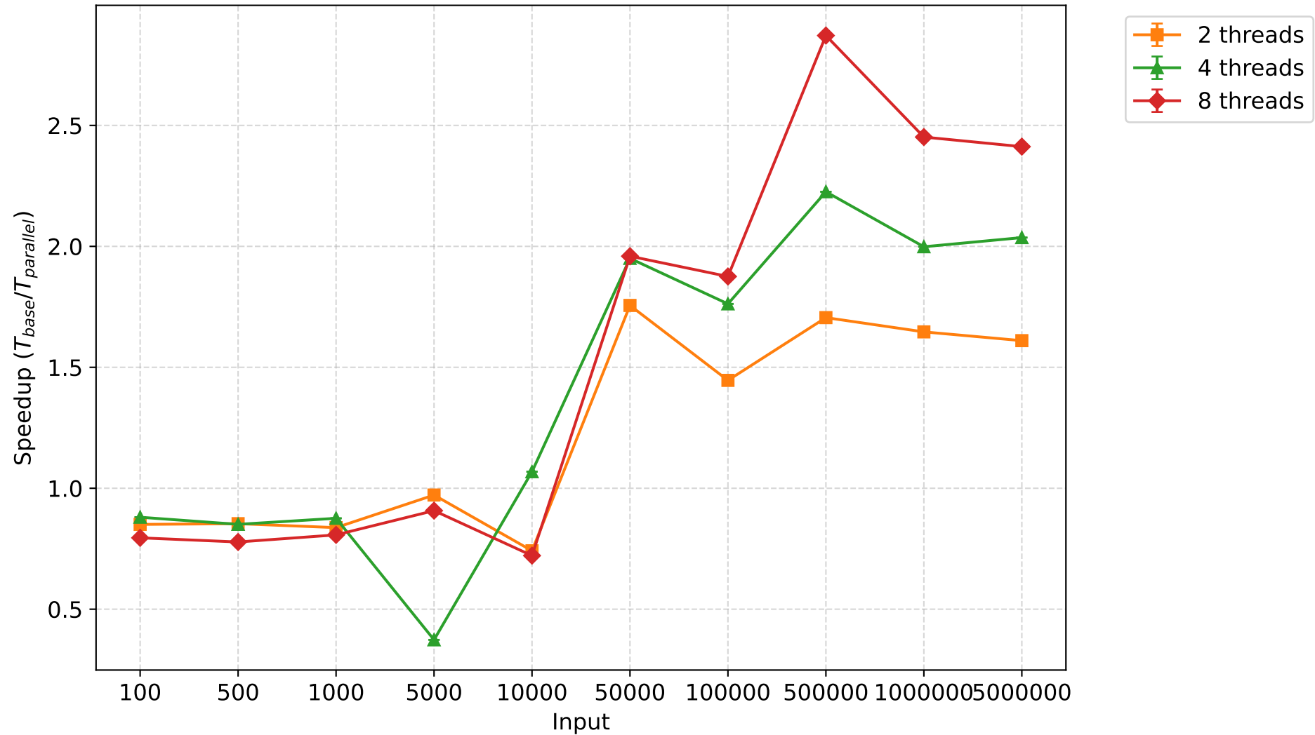
Speedup - mergesort (mean \pm 95% CI)
