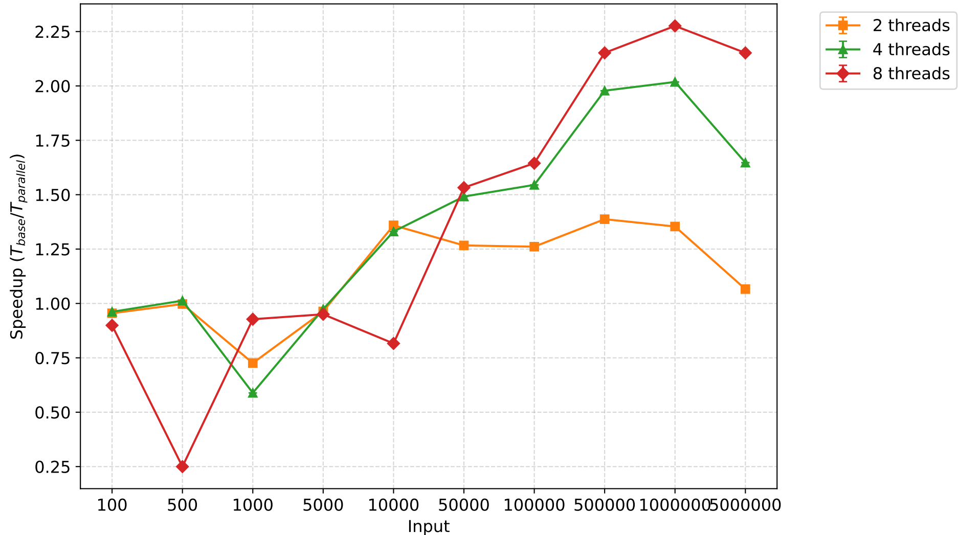
Speedup - shellsort (mean \pm 95% CI)
