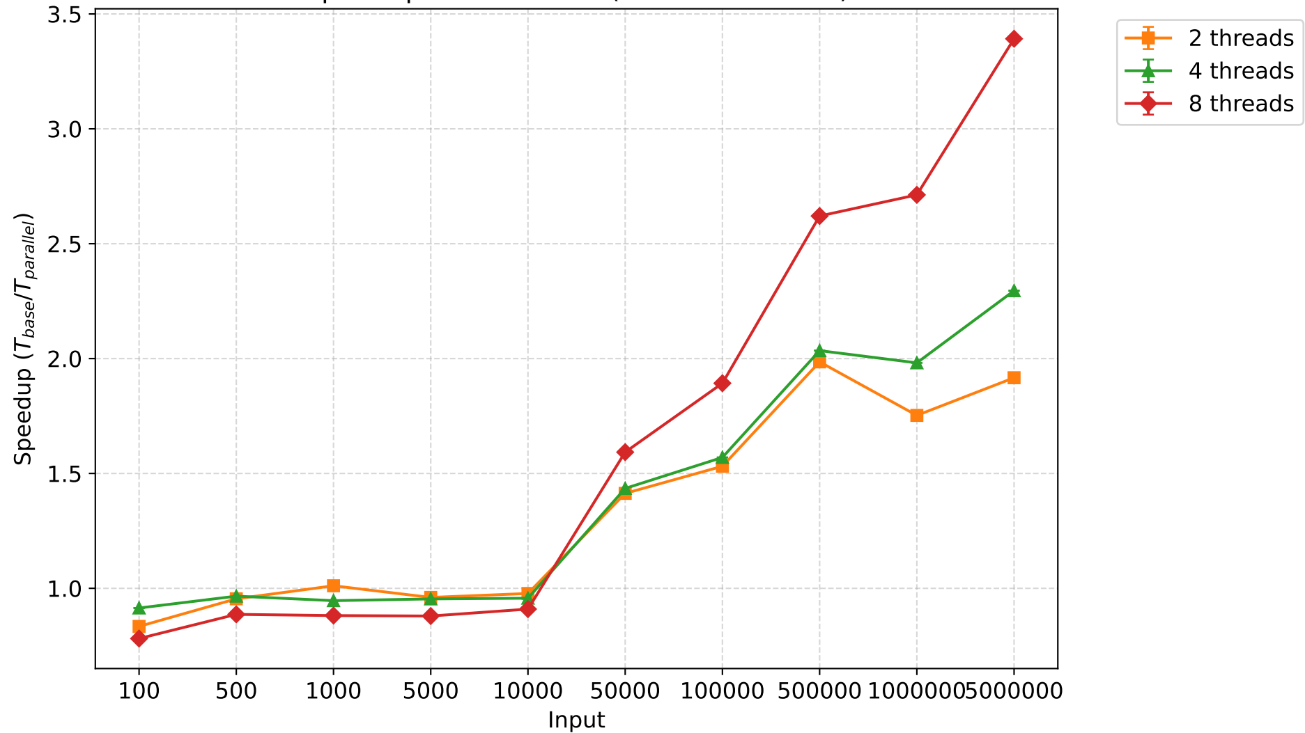
Speedup - smoothsort (mean \pm 95% CI)
