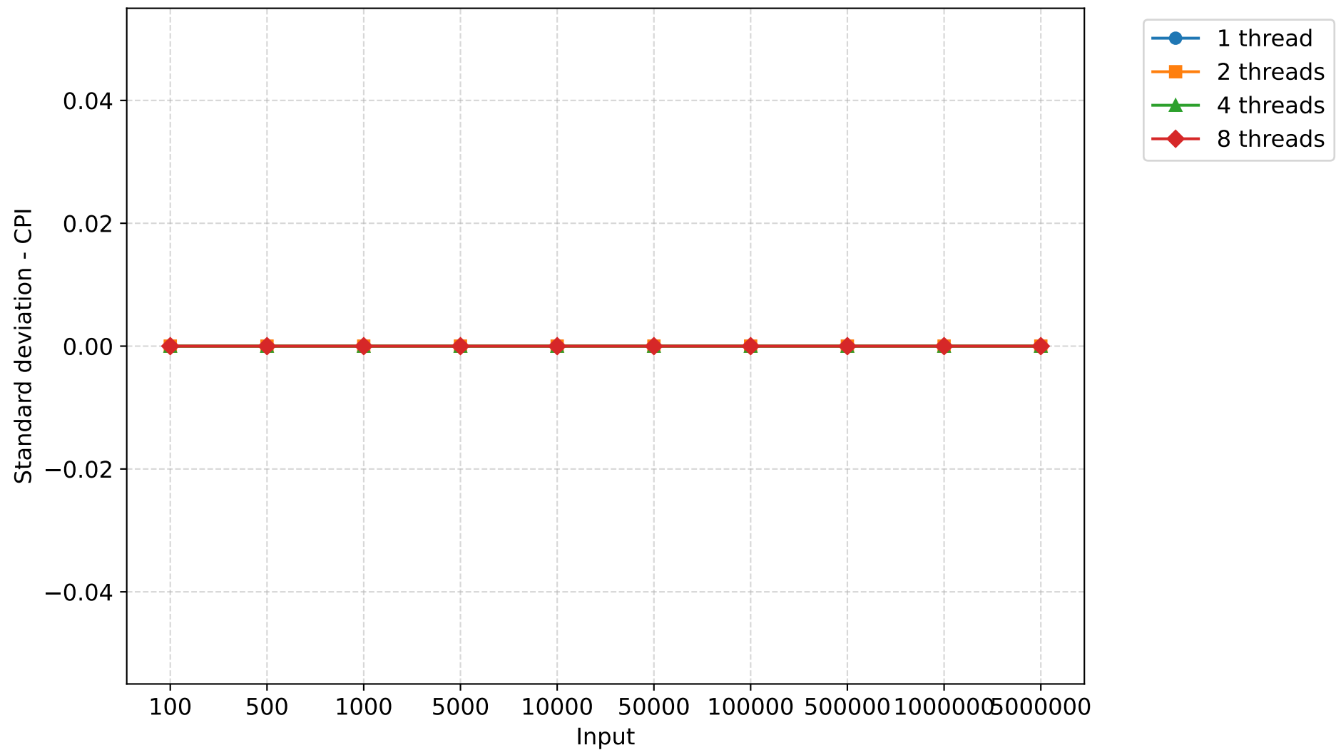
Standard deviation of CPI - combSORT
