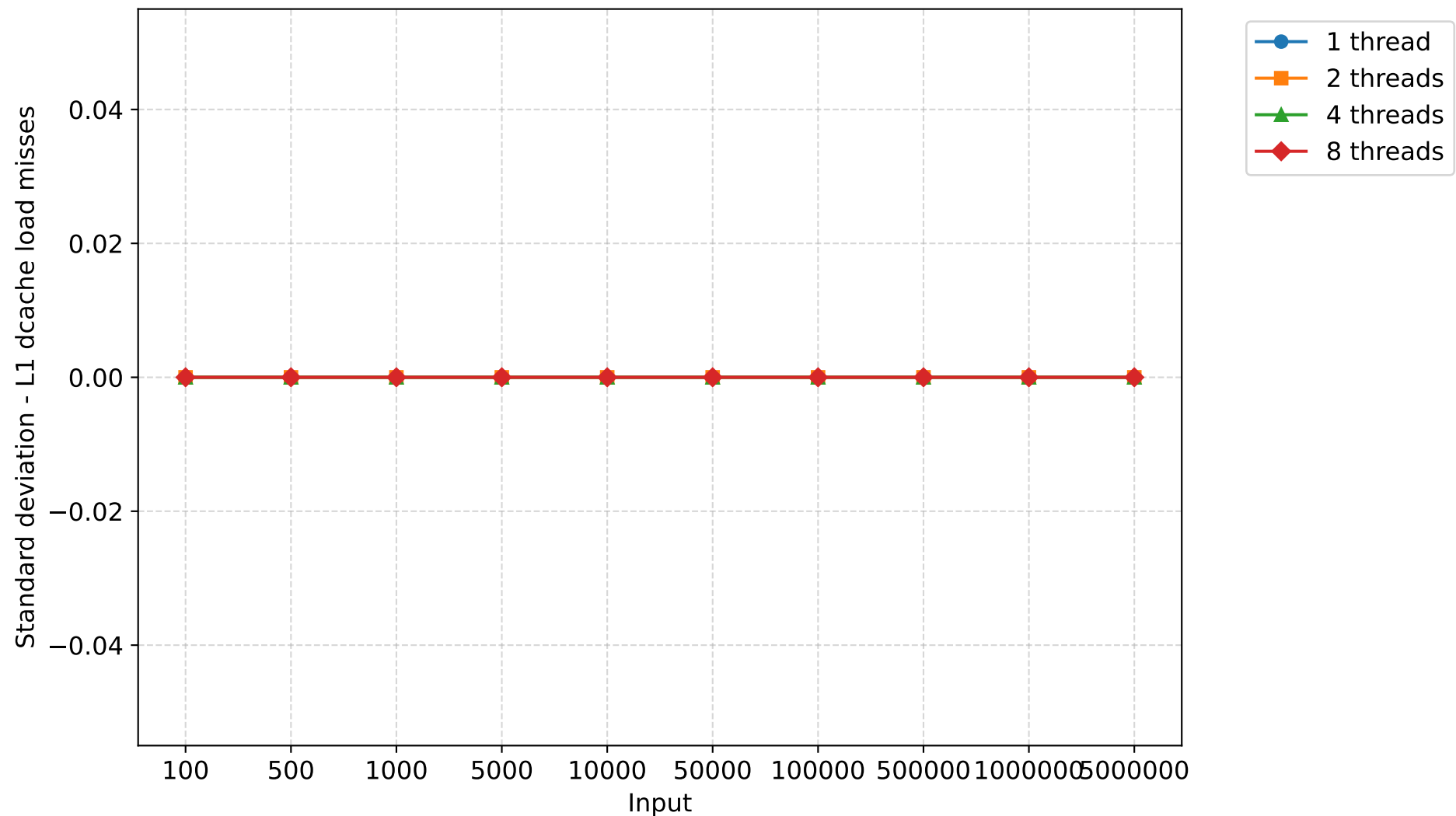
Standard deviation of L1 dcache load misses - smoothsort
