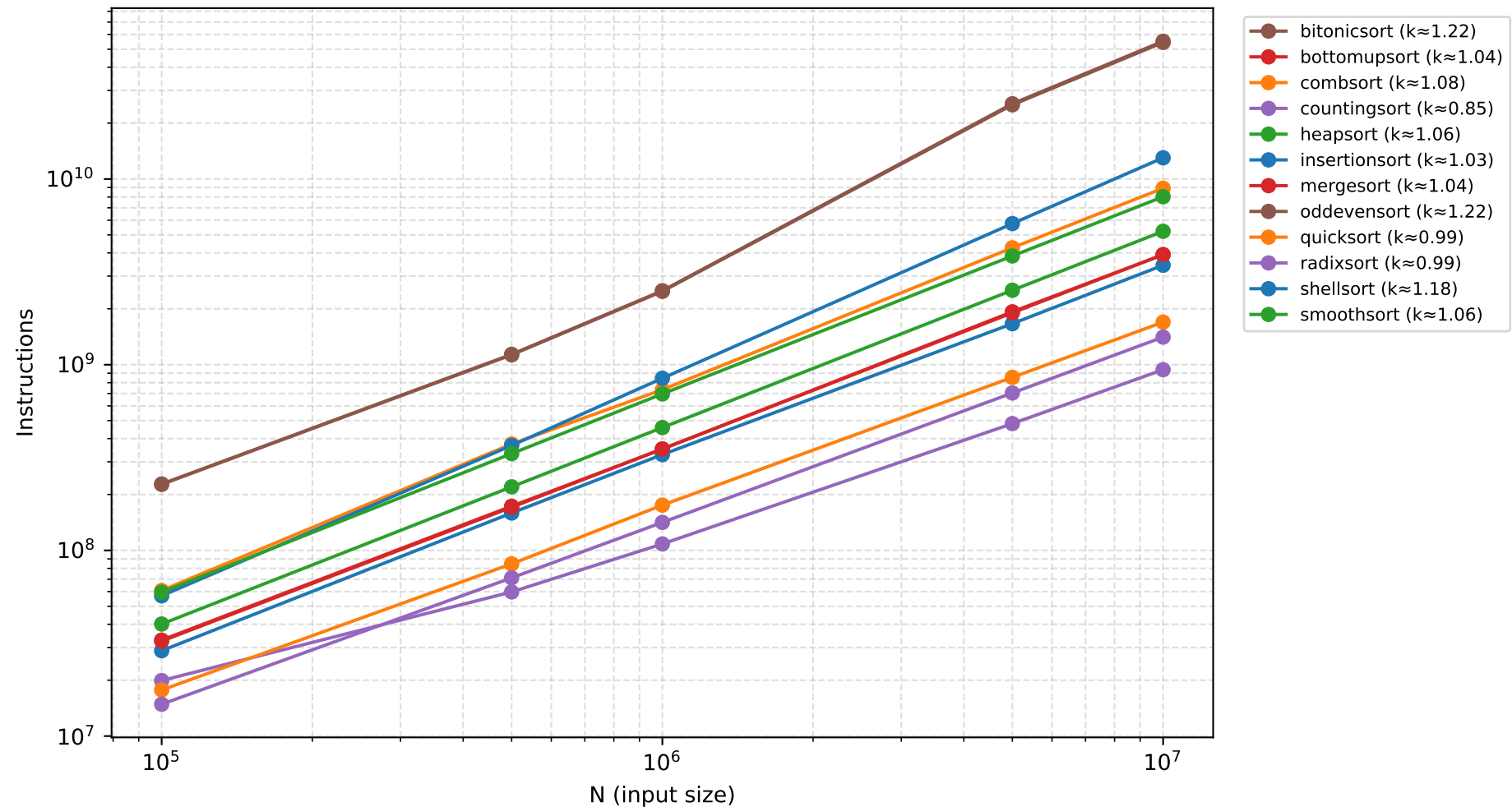
Empirical complexity — Instructions vs N (log-log, serial t1)
