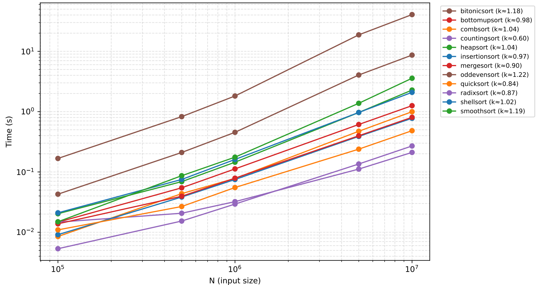
Empirical complexity — Time (s) vs N (log-log, serial t1)
