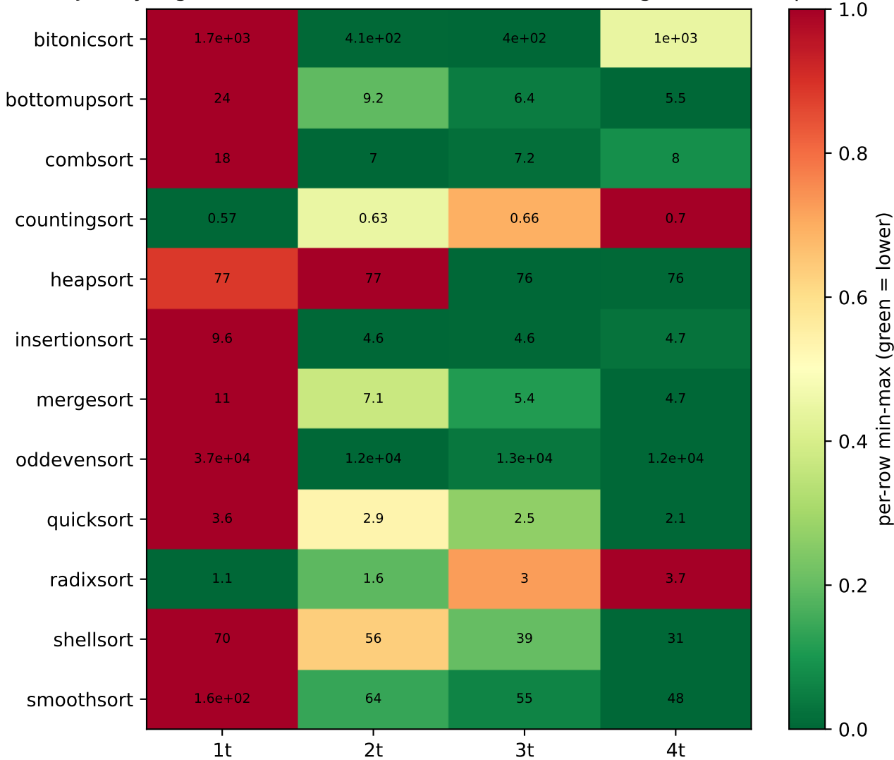
EDP (J·s) by algorithm imes threads ( N = 10000000 ) — green = best per row
