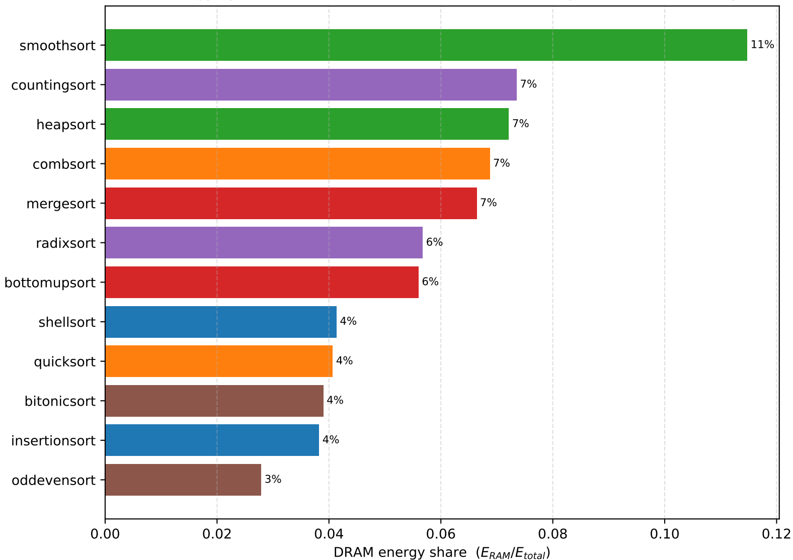
Share of energy spent in DRAM ( N = 10000000 , serial) — higher = more memory-bound
