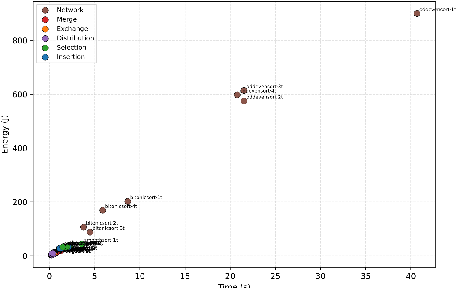
Energy-time trade-off ( N = 10000000 , all thread counts)
