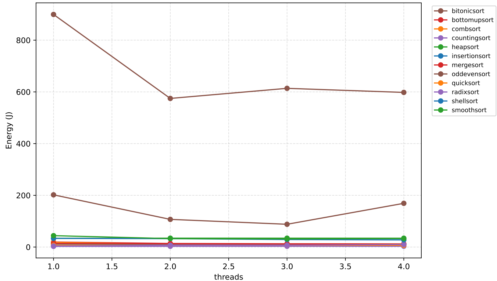
Total energy vs threads ( N = 100000000 ) — does not drop like time
