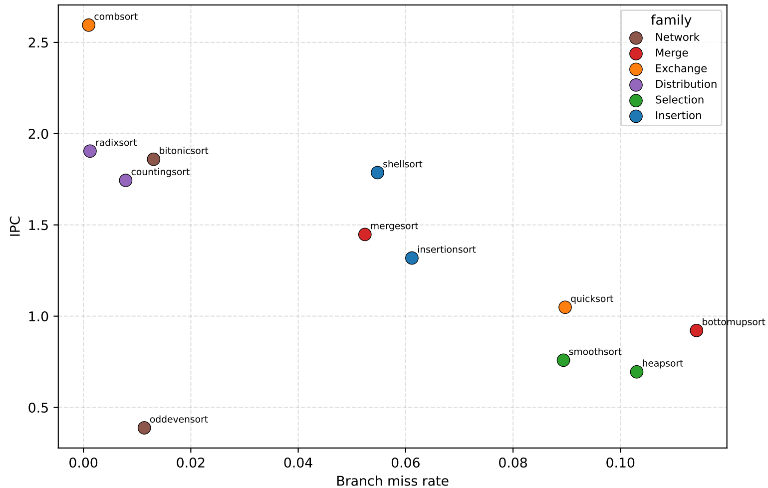
Microarchitecture fingerprint ( N = 10000000 , serial)
