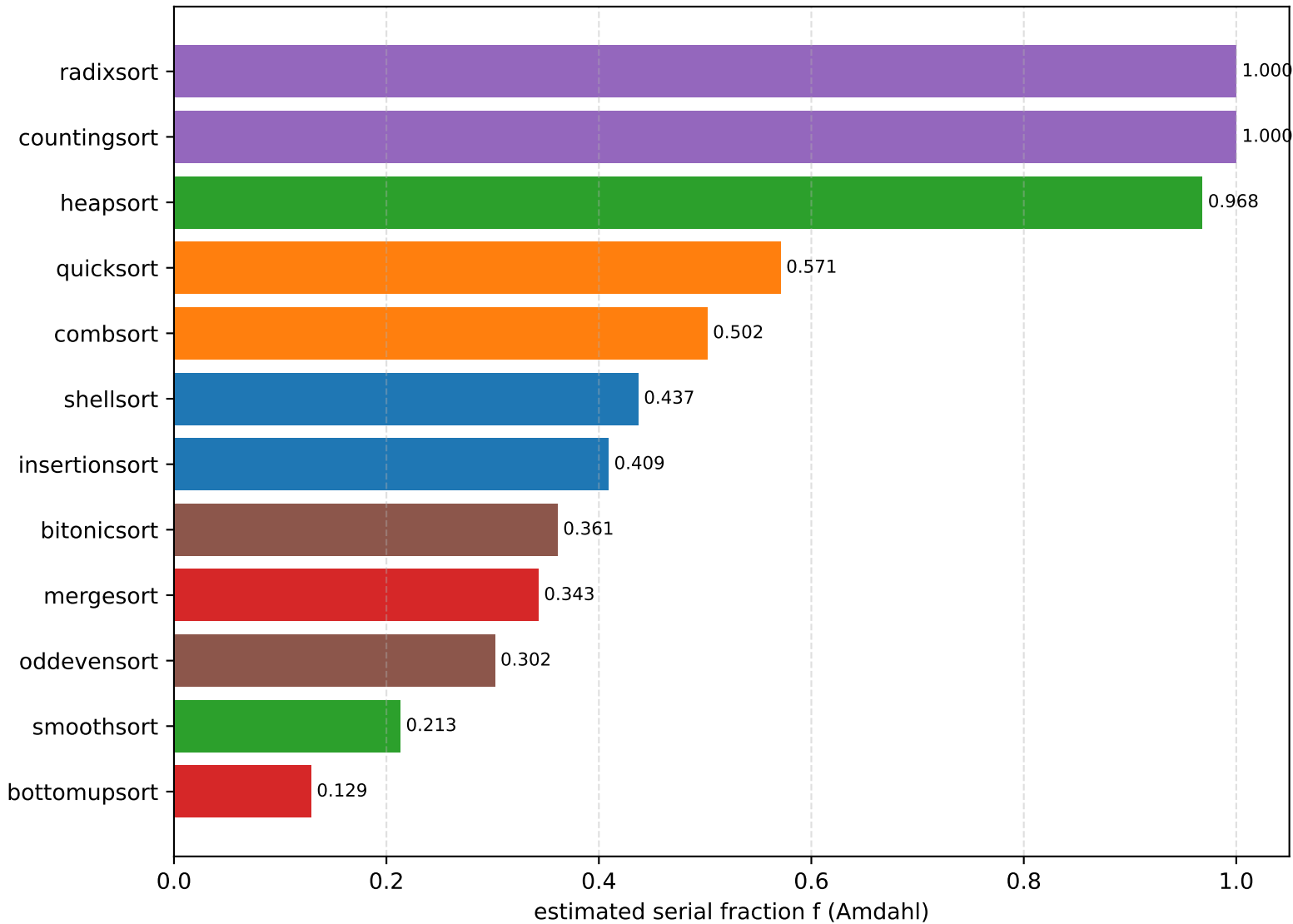
Serial fraction per algorithm ( N = 10000000 ) — lower f scales better
