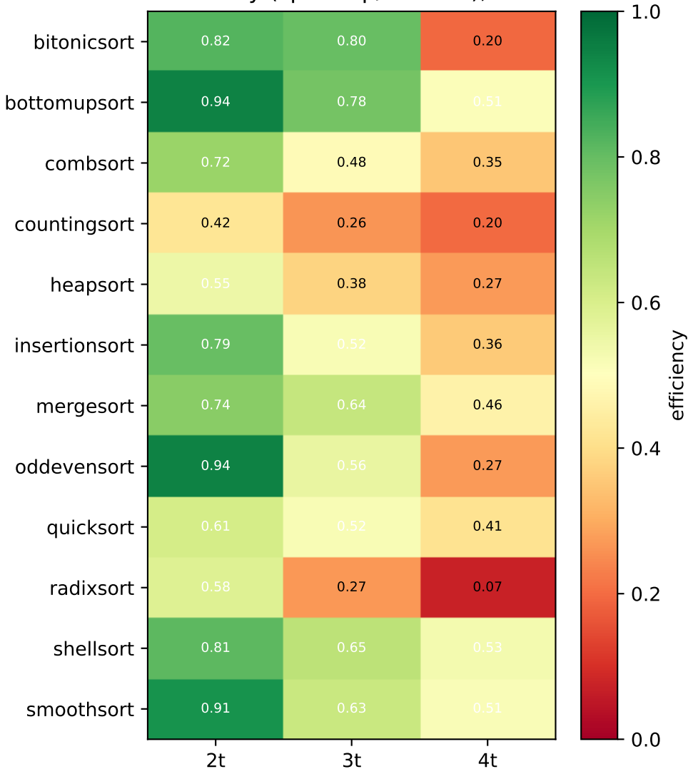
Parallel efficiency (speedup/threads), mean over N
