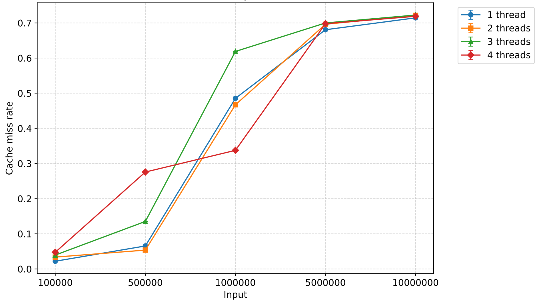
Cache miss rate - bottomupsort (mean \pm 95% CI)
