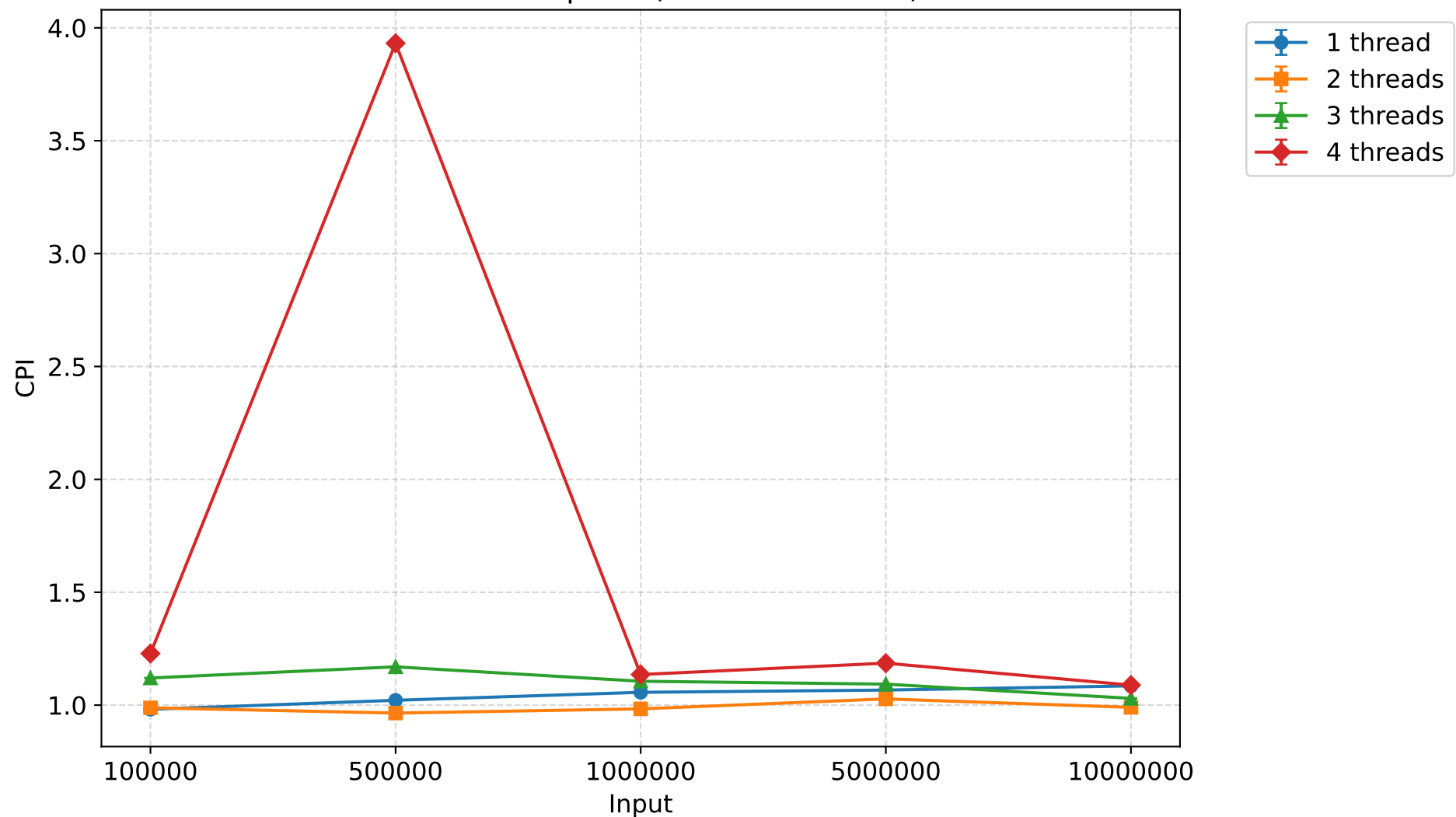
CPI - bottomupsort (mean \pm 95% CI)
