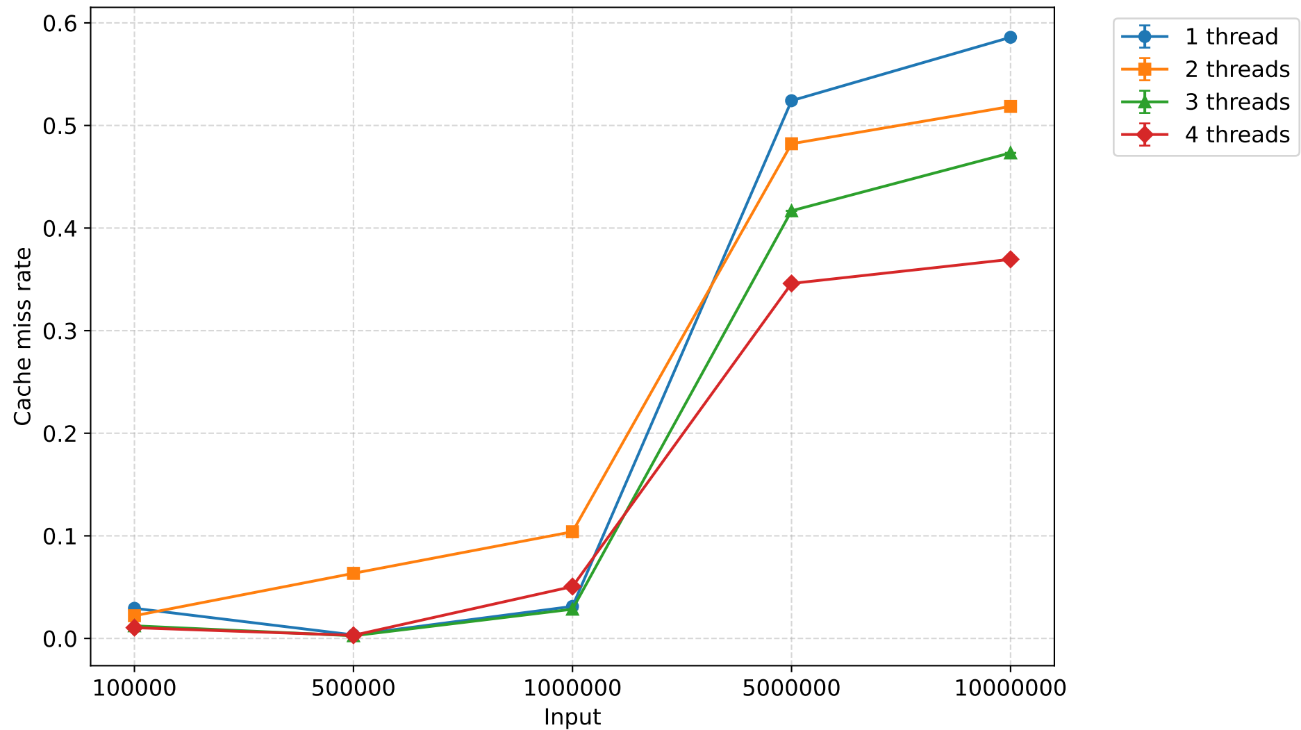
Cache miss rate - combSORT (mean \pm 95% CI)
