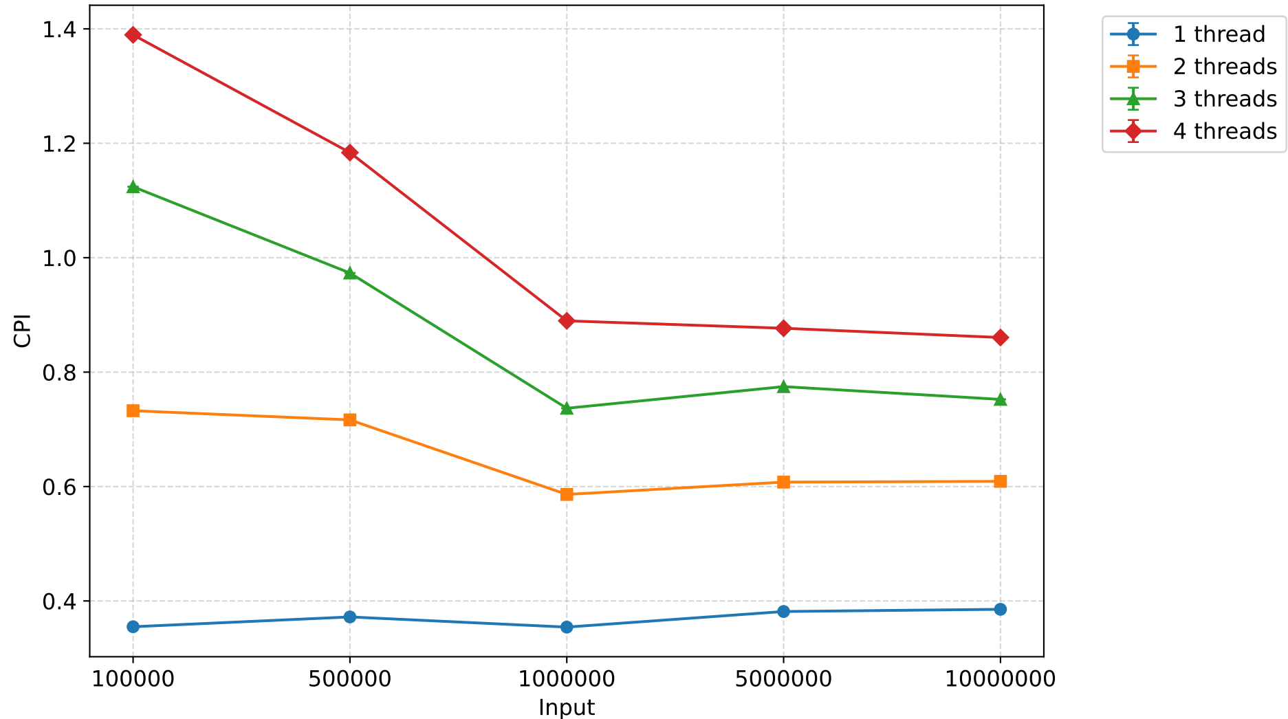
CPI - combsort (mean \pm 95% CI)
