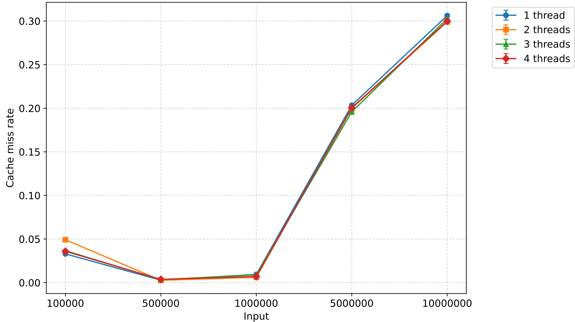
Cache miss rate - heapsort (mean \pm 95% CI)
