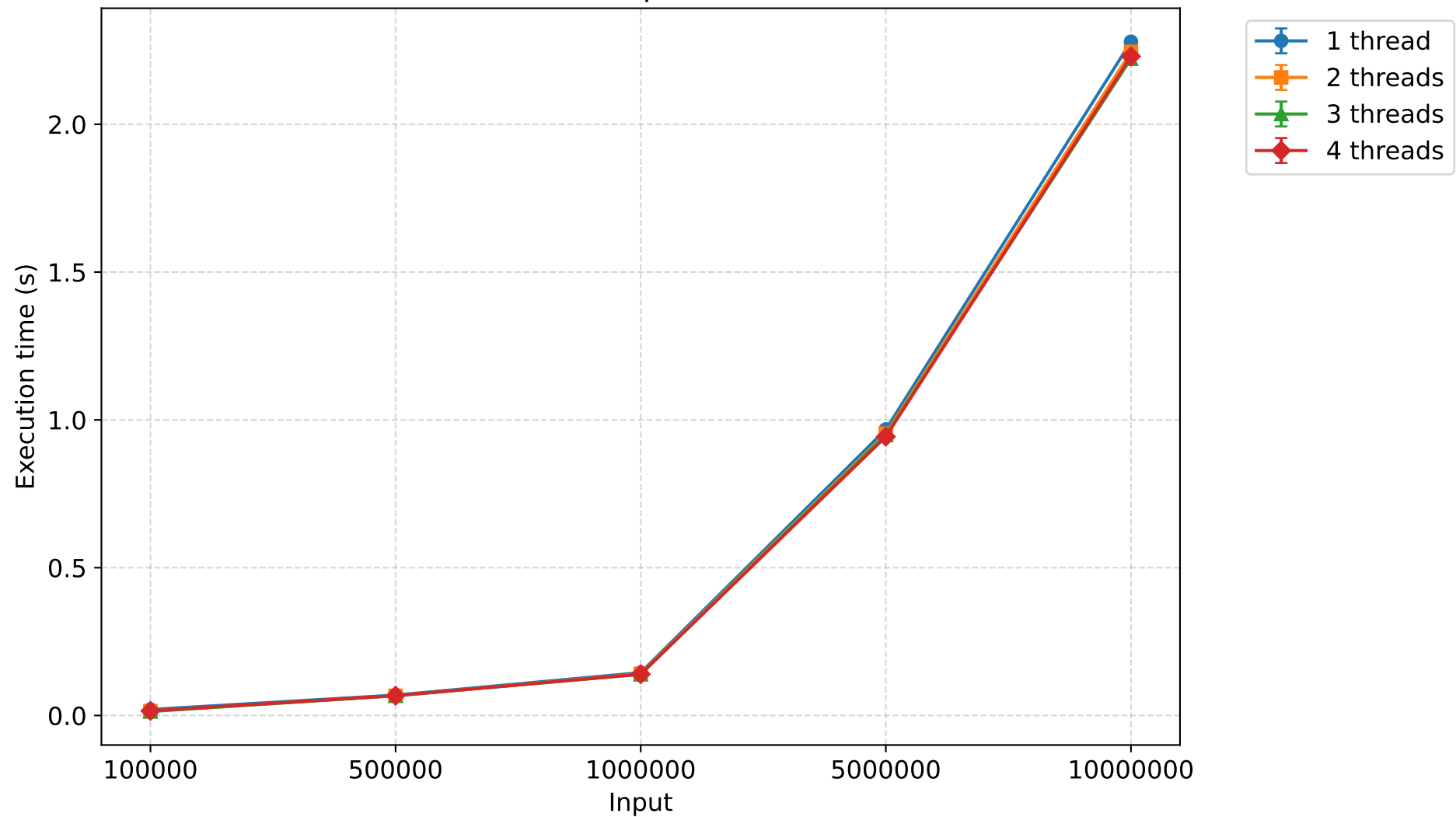
Execution time (s) - heapsort (mean \pm 95% CI)
