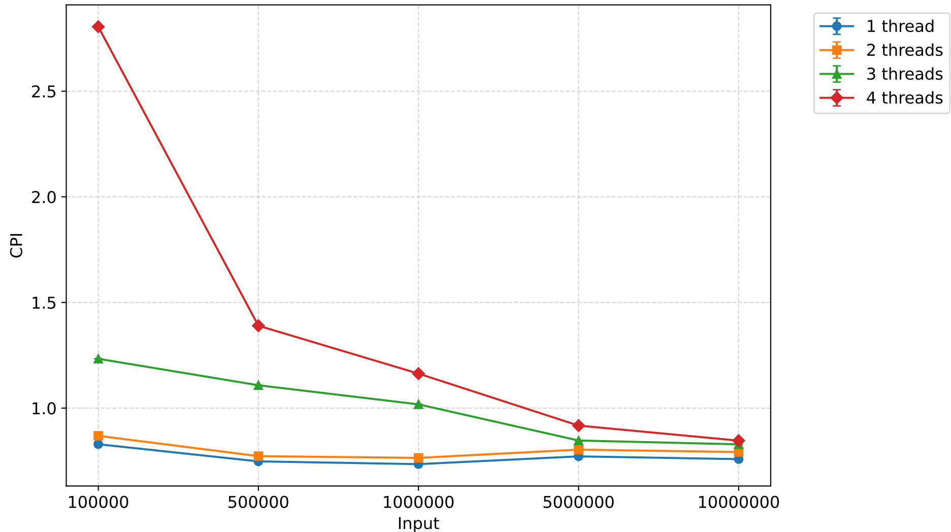
CPI - insertionsort (mean \pm 95% CI)
