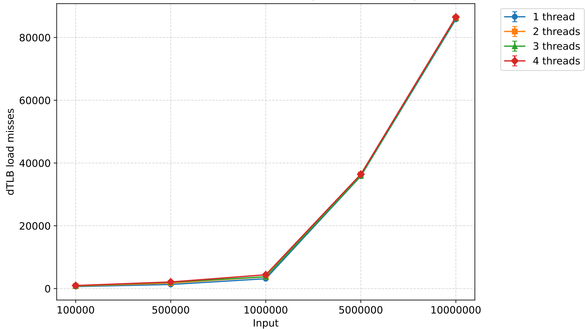
dTLB load misses - insertionsort (mean \pm 95% CI)
