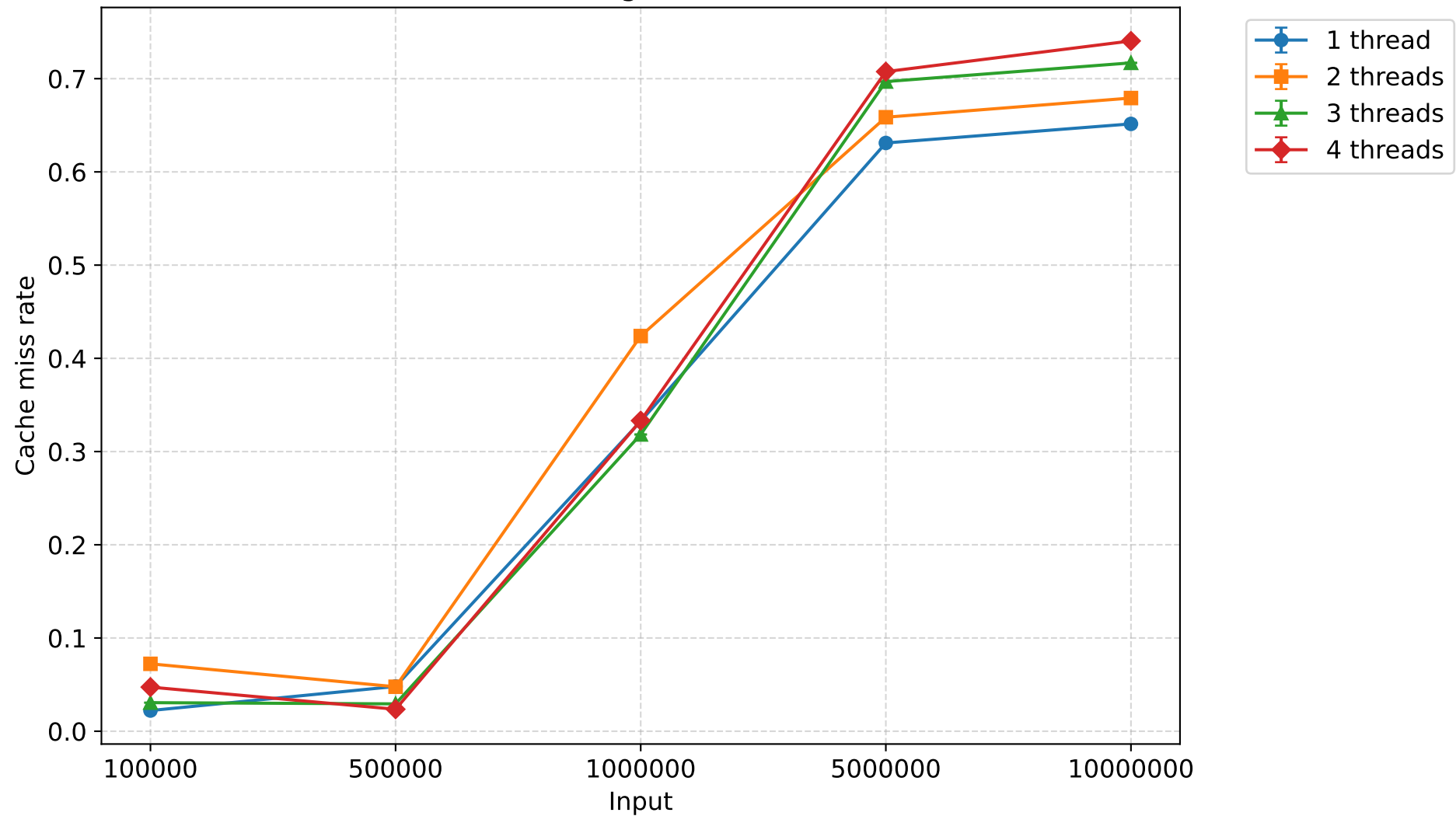
Cache miss rate - mergesort (mean \pm 95% CI)
