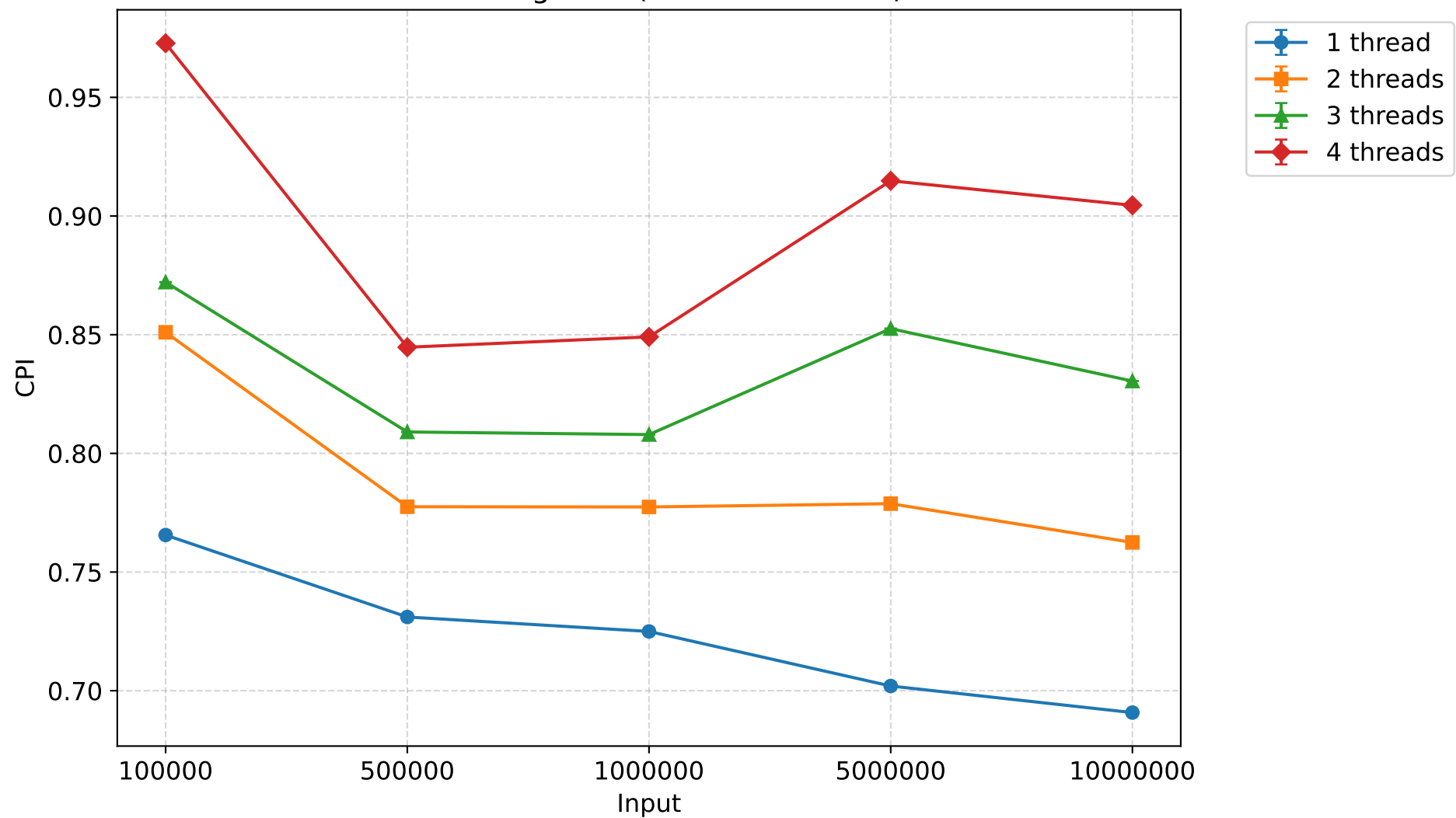
CPI - mergesort (mean \pm 95% CI)
