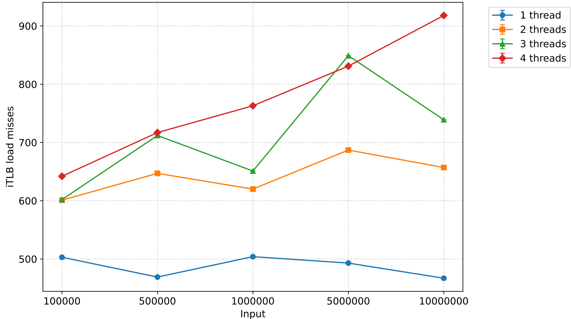
iTLB load misses - quicksort (mean \pm 95% CI)
