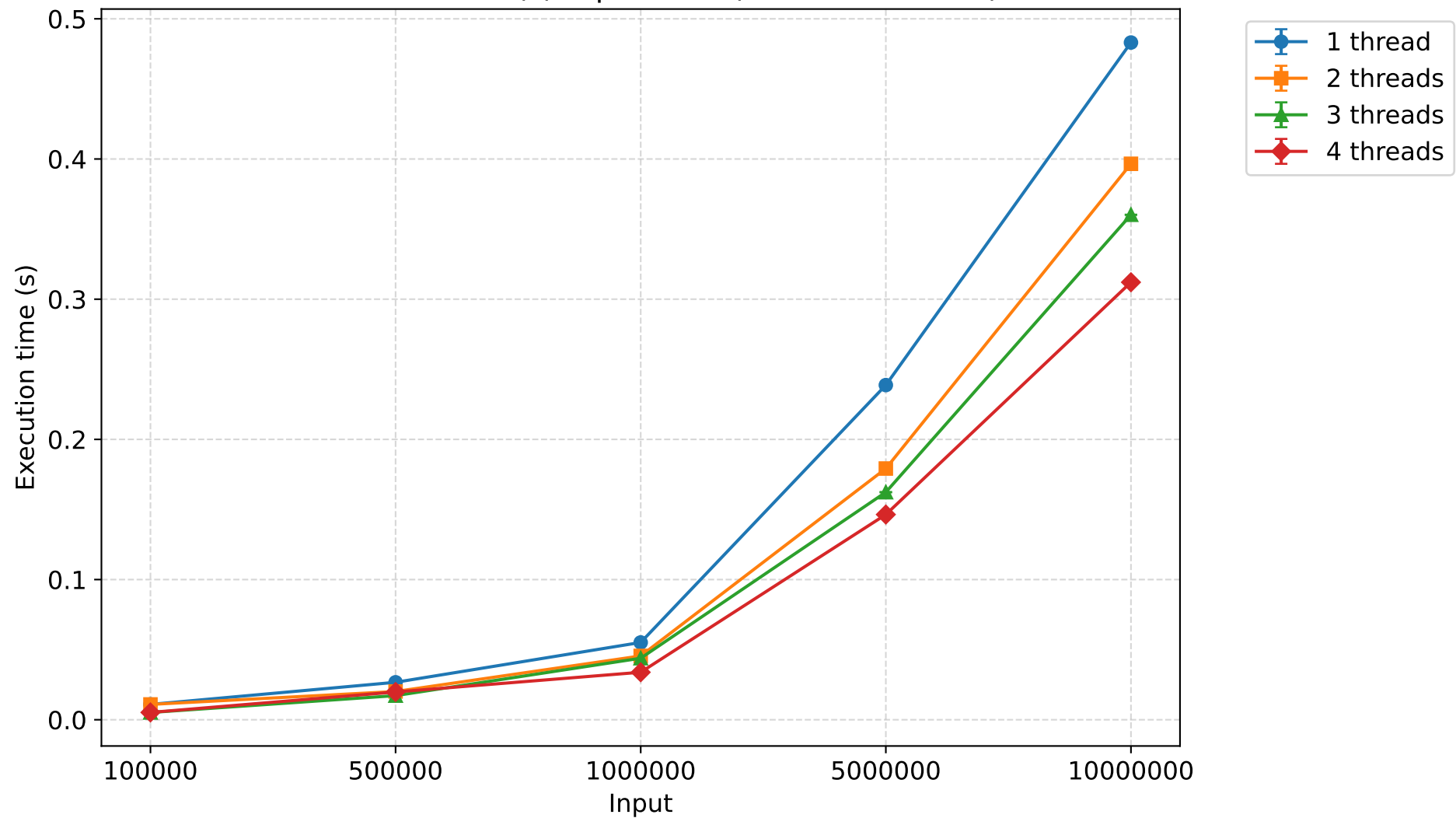
Execution time (s) - quicksort (mean \pm 95% CI)
