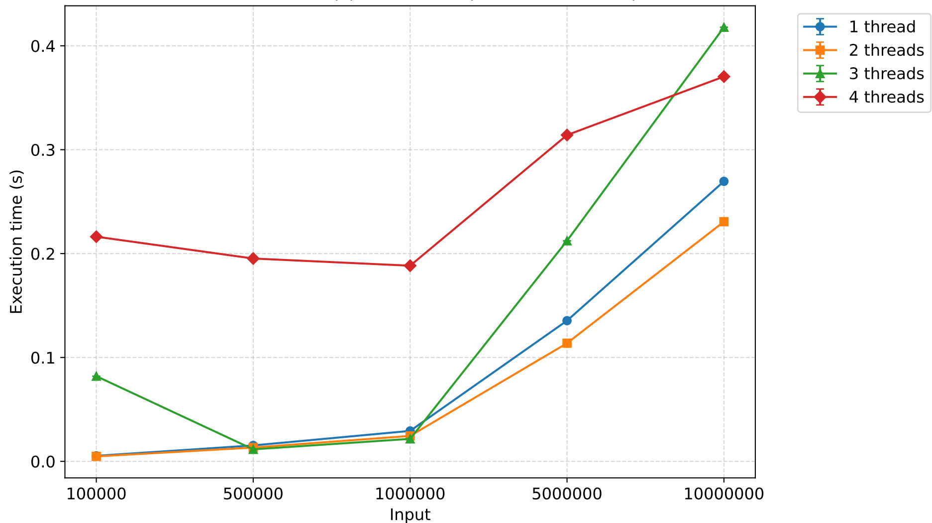
Execution time (s) - radixsort (mean \pm 95% CI)
