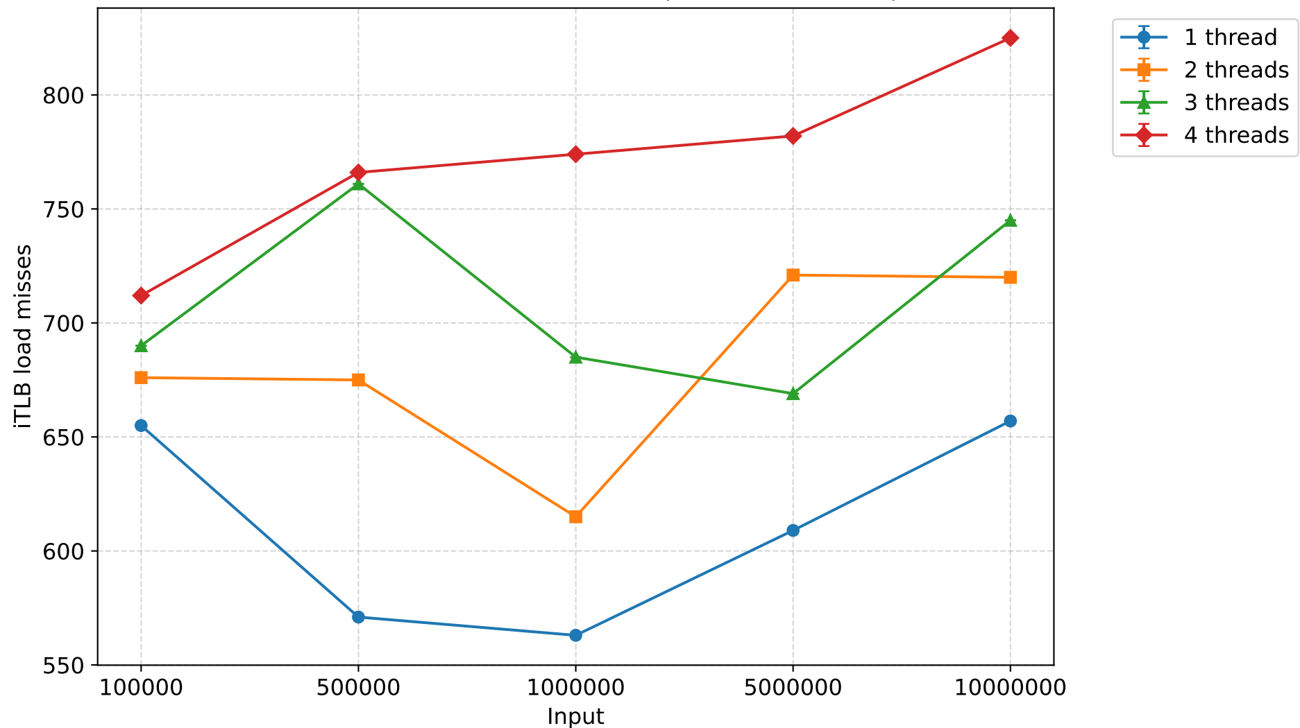
iTLB load misses - smoothsort (mean \pm 95% CI)
