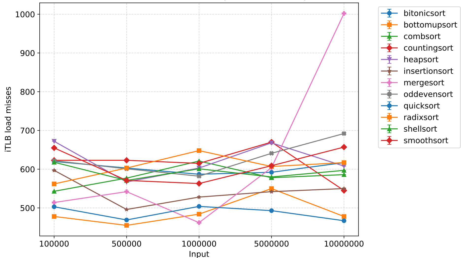
iTLB load misses - 1 thread (mean \pm 95% CI)
