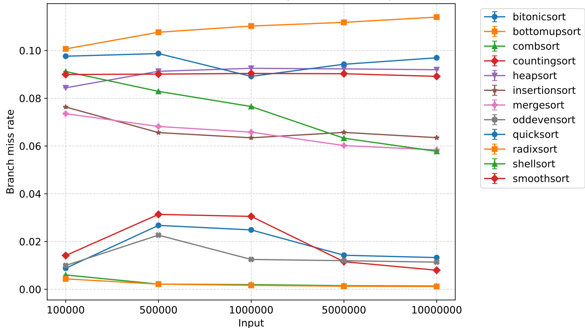
Branch miss rate - 3 threads (mean \pm 95% CI)
