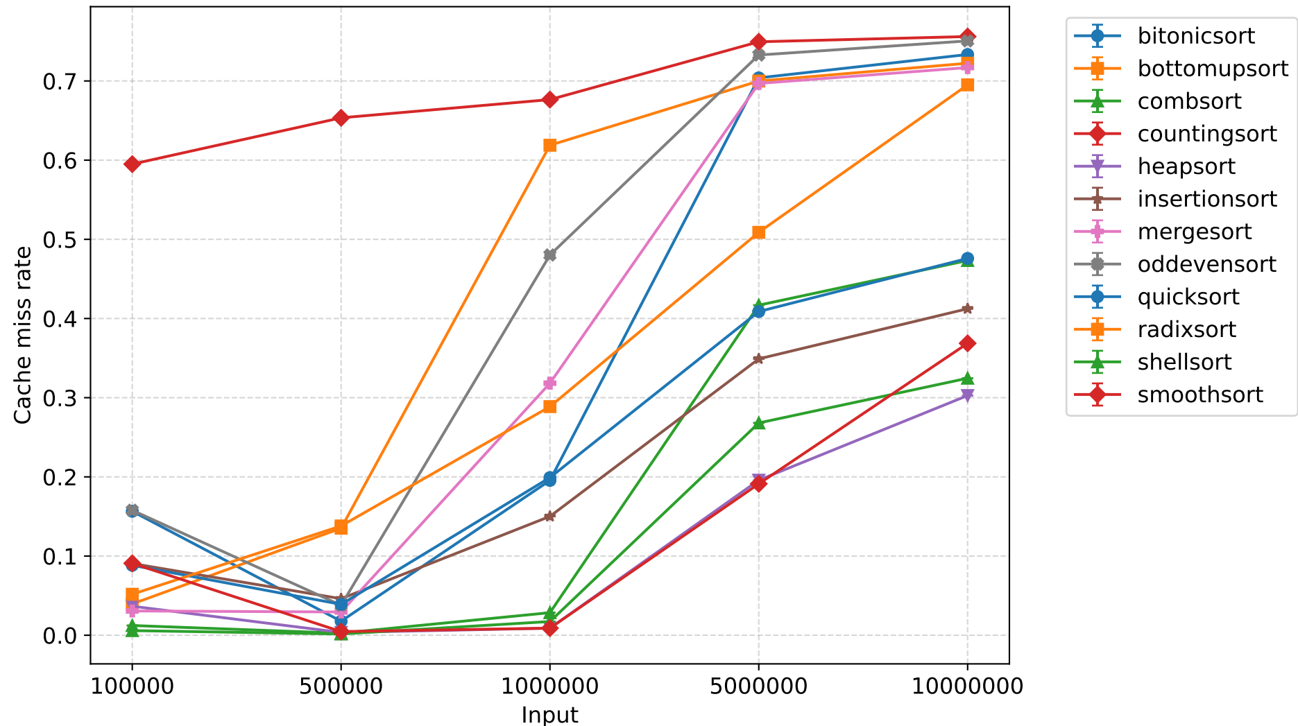
Cache miss rate - 3 threads (mean \pm 95% CI)
