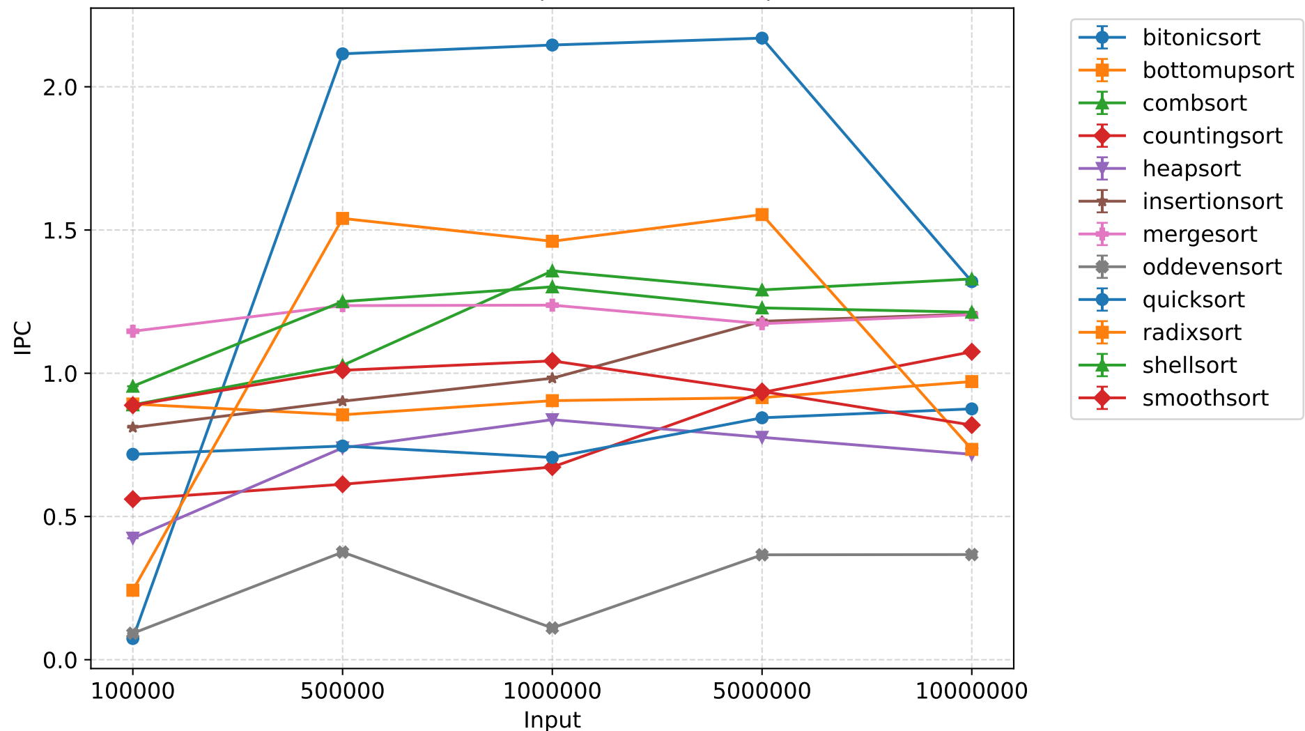
IPC - 3 threads (mean \pm 95% CI)
