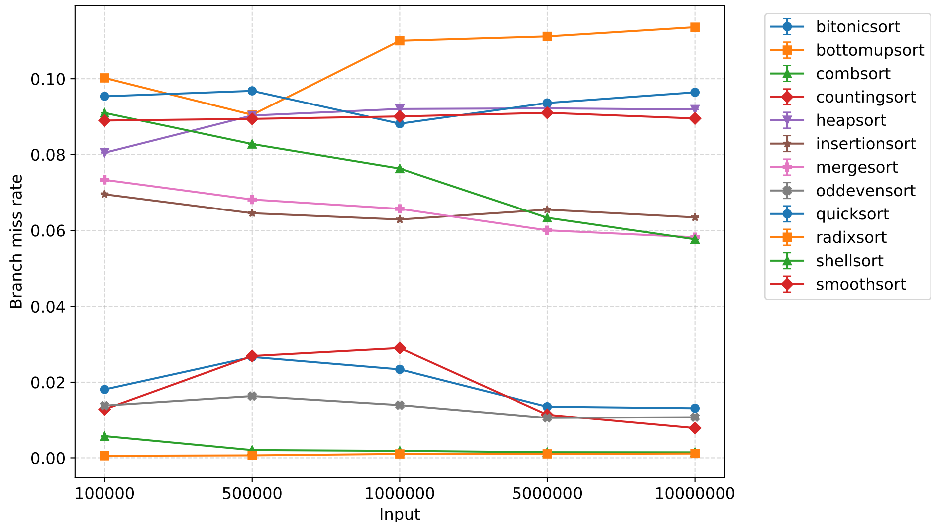
Branch miss rate - 4 threads (mean \pm 95% CI)
