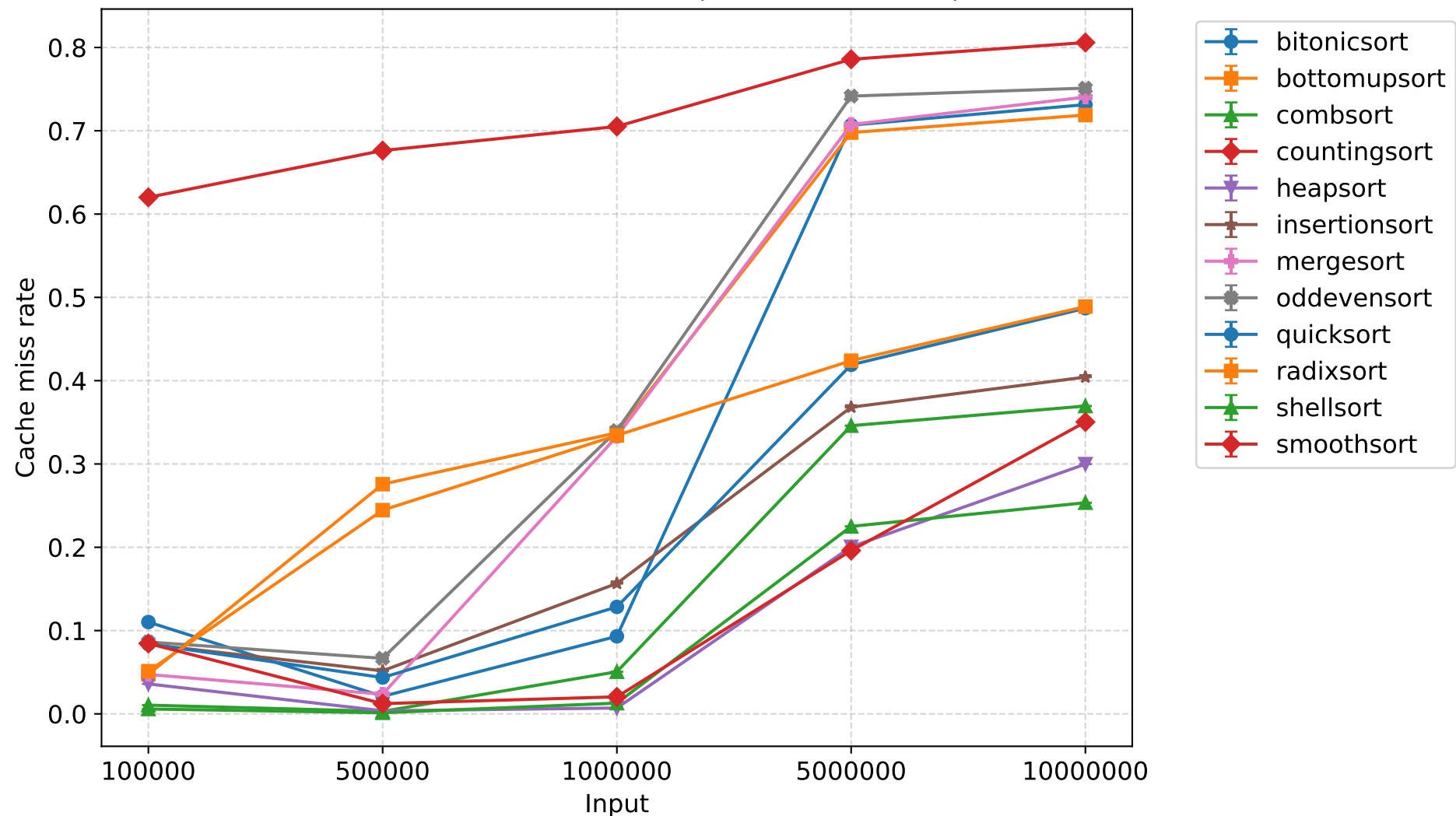
Cache miss rate - 4 threads (mean \pm 95% CI)
