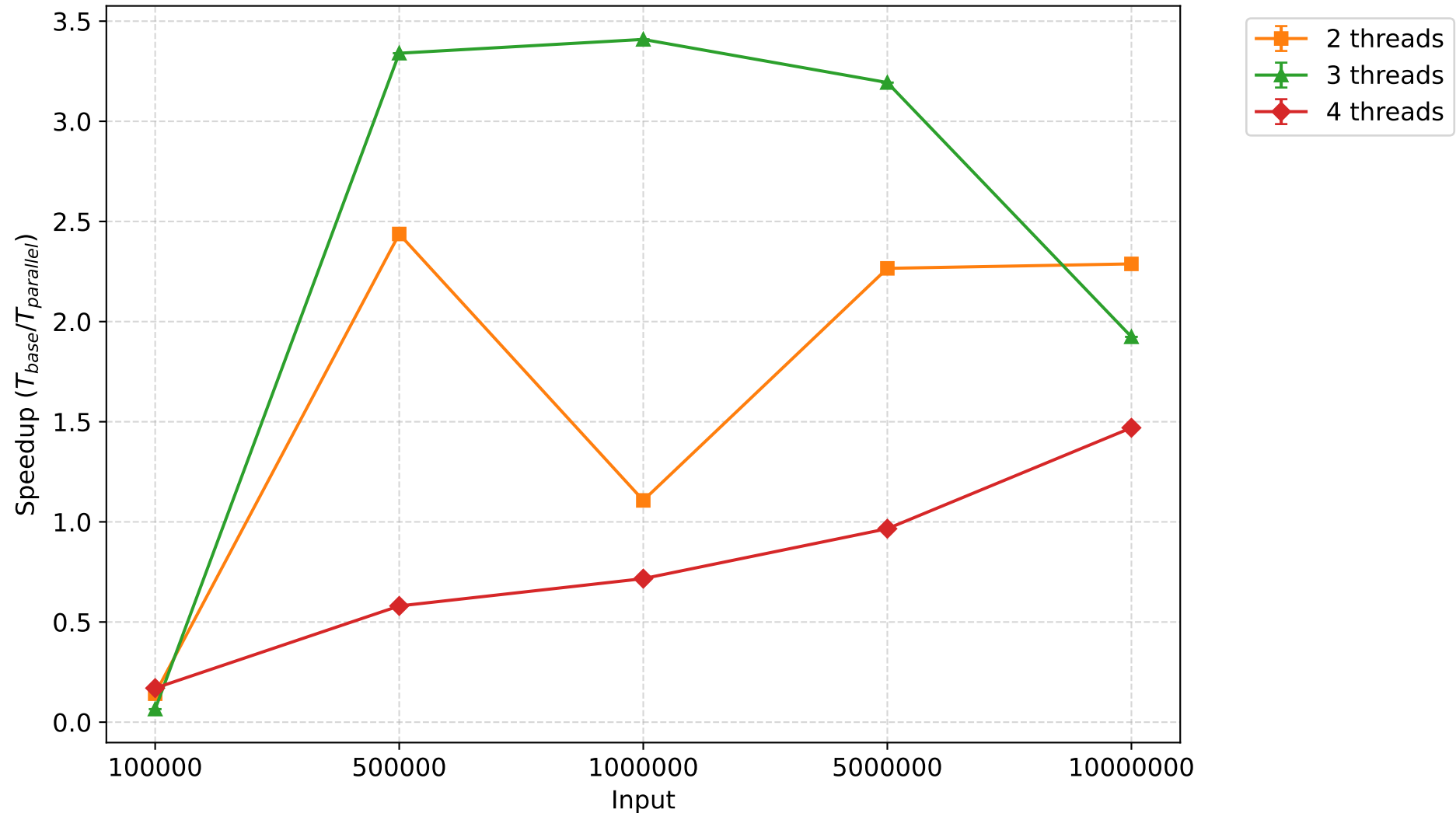
Speedup - bitonicsort (mean \pm 95% CI)
