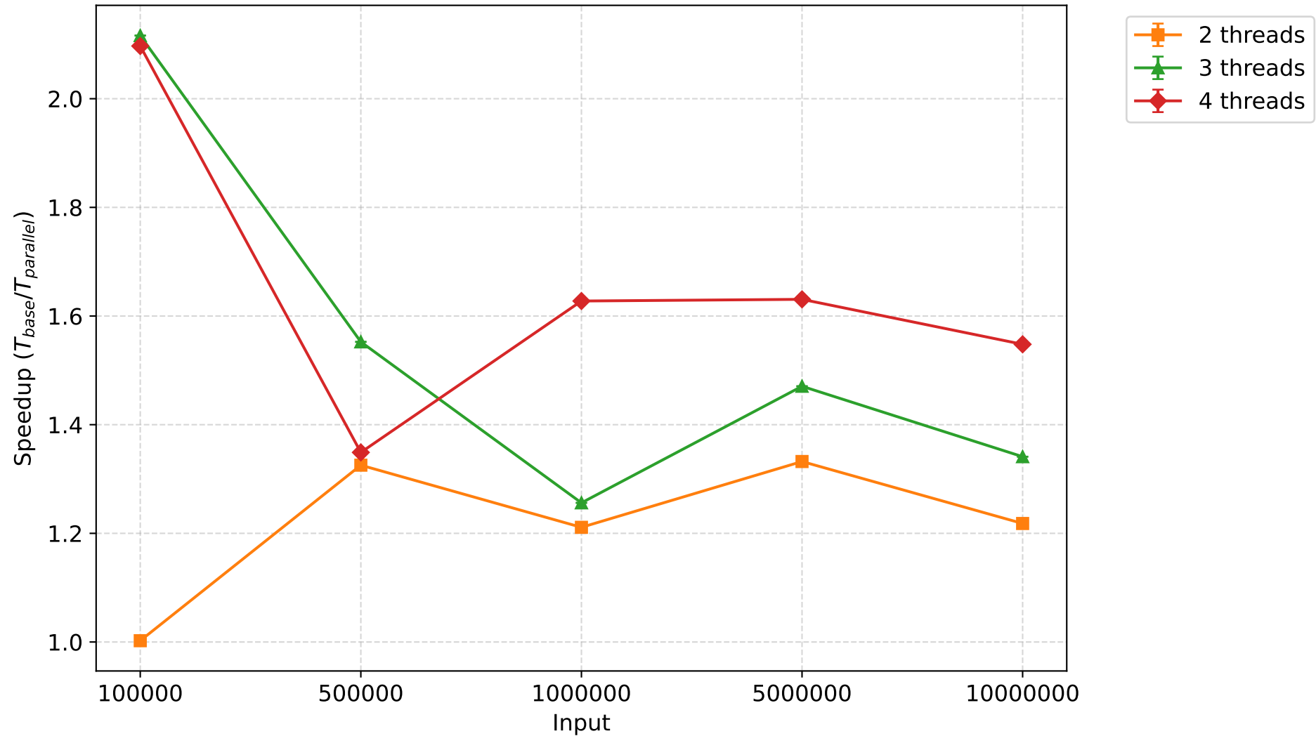
Speedup - quicksort (mean \pm 95% CI)
