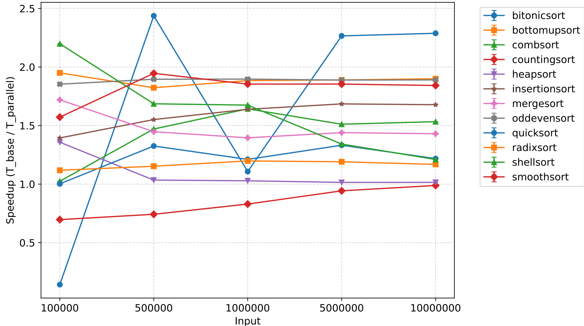
Speedup - 2 threads (mean +- 95% CI)
