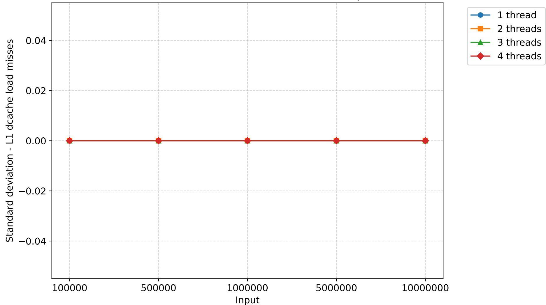
Standard deviation of L1 dcache load misses - quicksort
