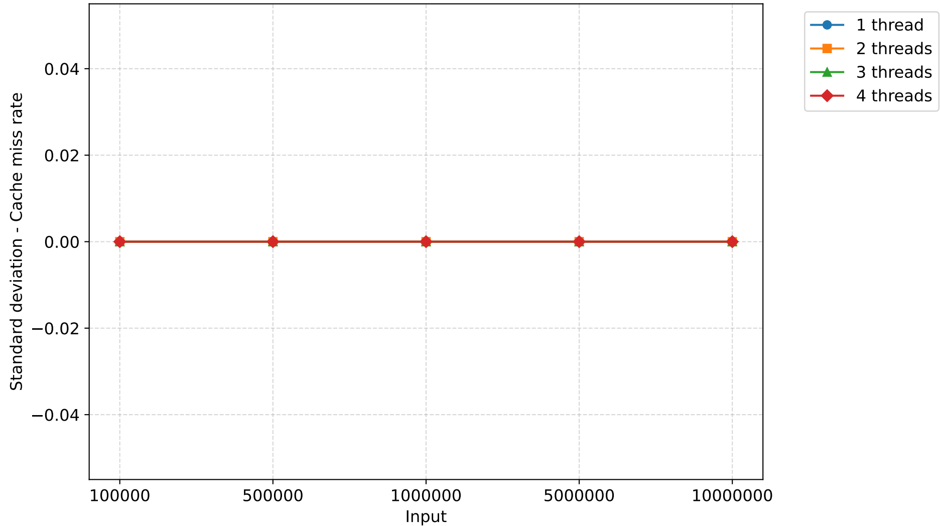
Standard deviation of Cache miss rate - shellsort
