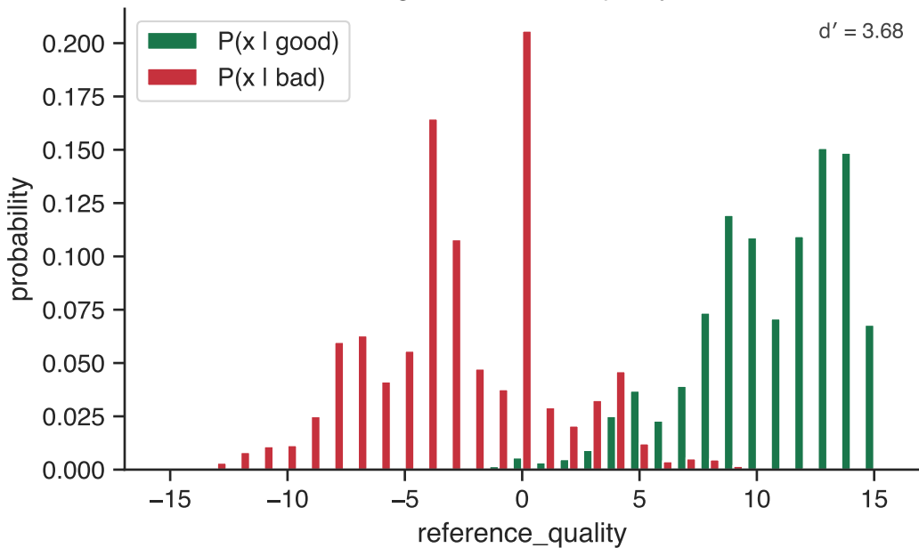
Signal: reference_quality
