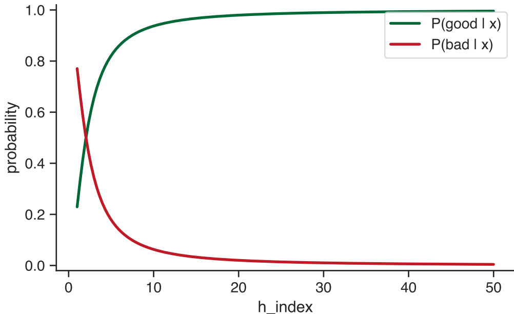
P(\text{state} \mid x) - h\_index
