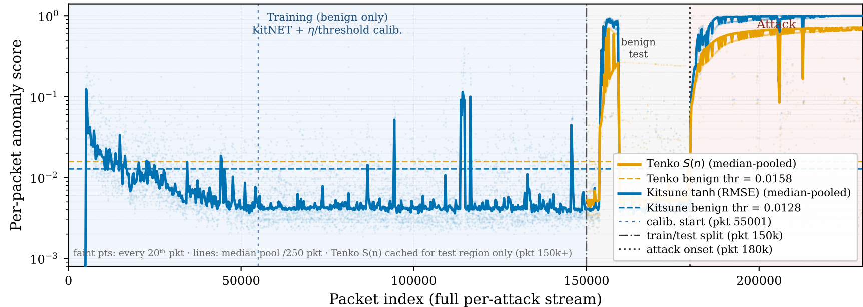
Tenko vs Kitsune anomaly score, full stream — MITM ARP Spoofing (CICIoT2023)
