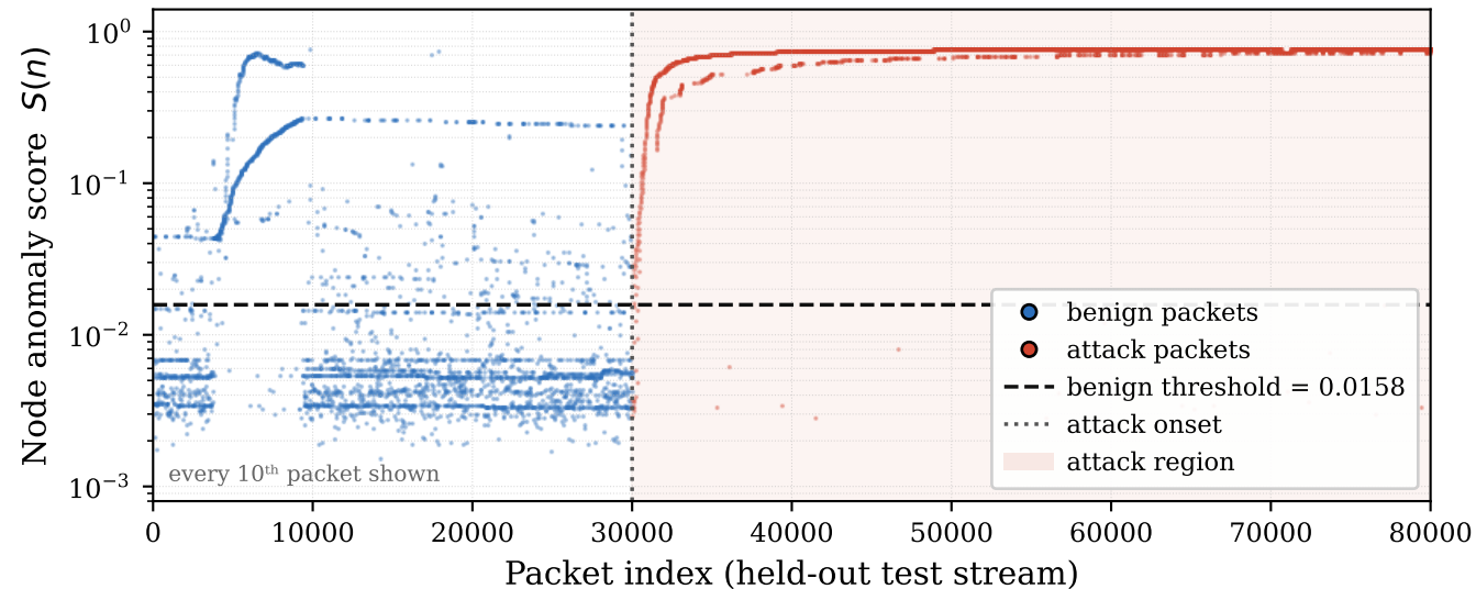
Tenko (node-aggregated score) — DoS SYN Flood (CICIoT2023)
