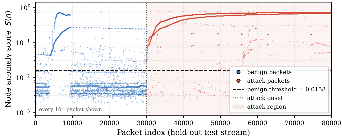
Tenko (node-aggregated score) — MITM ARP Spoofing (CICIoT2023)
