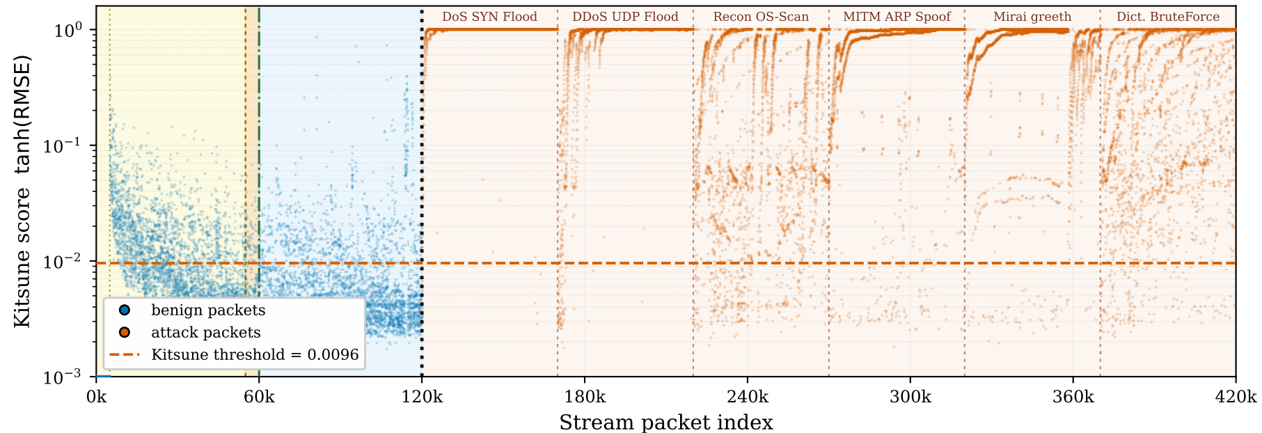
Kitsune anomaly score — CICIoT2023 mixed stream (single-tanh)
