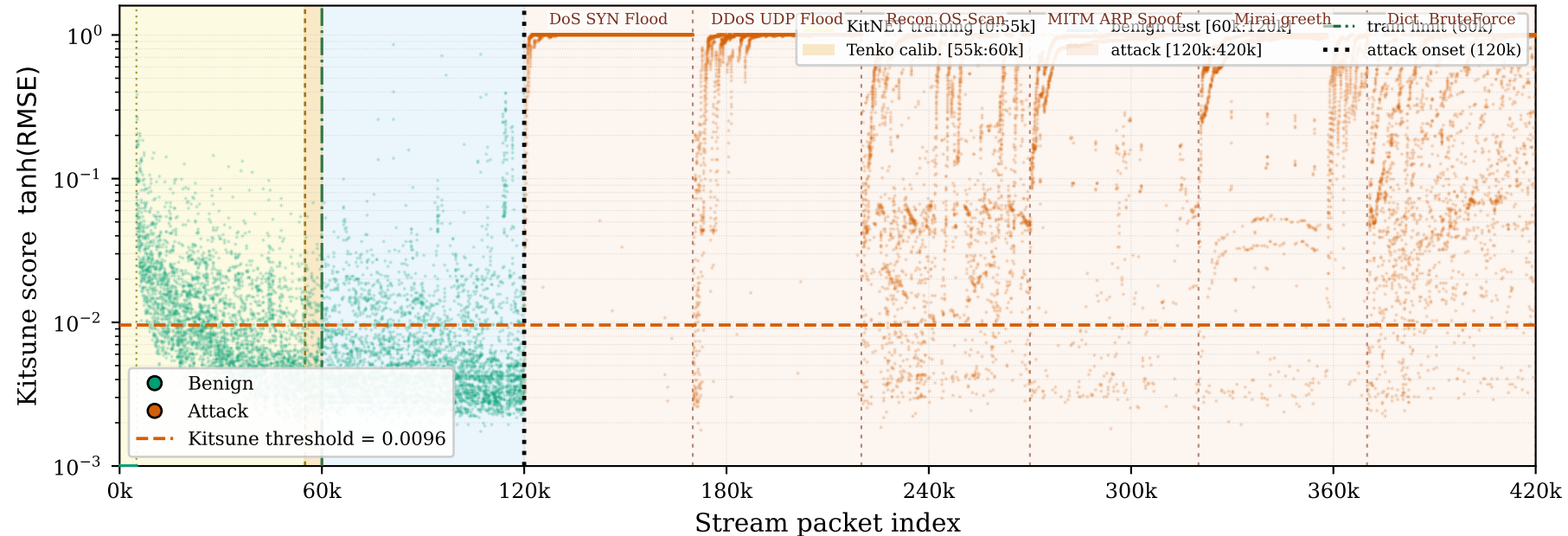
Kitsune anomaly score (label-colored) — CICIoT2023 mixed stream
