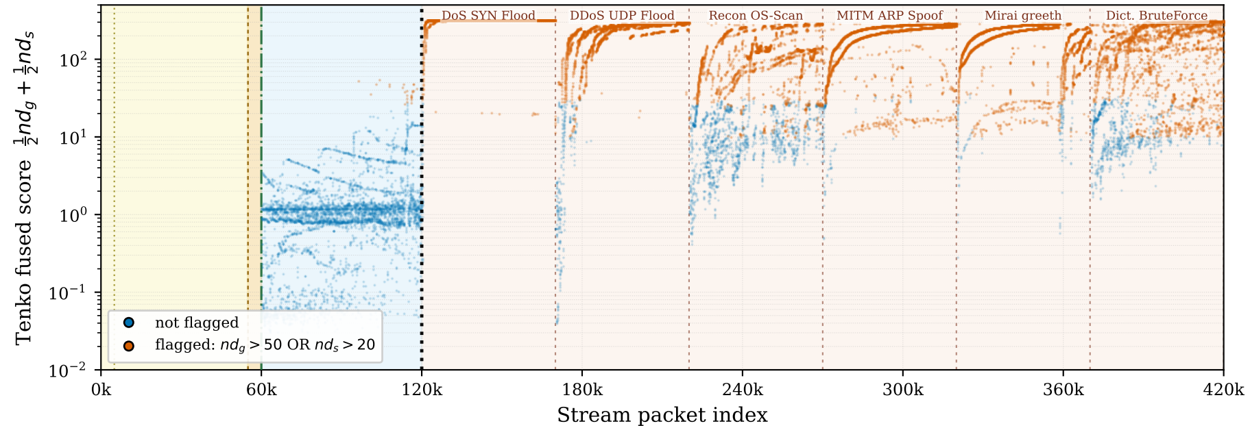
Tenko fused anomaly score — CICIoT2023 mixed stream (committed \eta = 50/20 )
